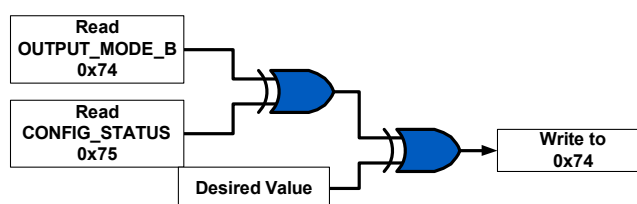
Figure 43. Setting OUTPUT_MODE_B Register
