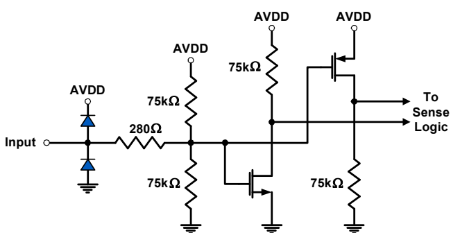
Figure 46. Tri-Level Digital Inputs
