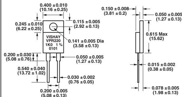
FIGURE 4 - VPR220 DIMENSIONS in inches (millimeters)
