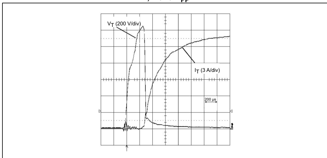
Figure 18. Current and voltage of the ACS120 during IEC 61000-4-5 standard test with R, L and V_{pp}
