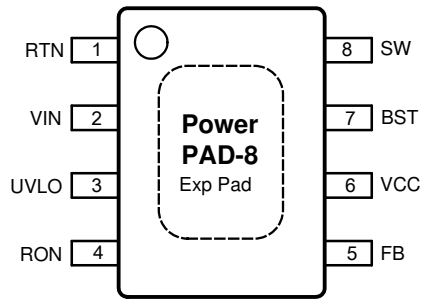
Connect Exposed Pad to RTN Figure 5-1. DDA Package 8-Pin SO PowerPAD Top View
