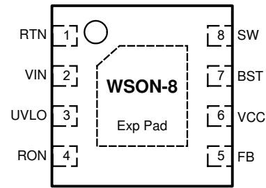
Connect Exposed Pad to RTN Figure 5-2. NGU Package 8-Pin WSON Top View
