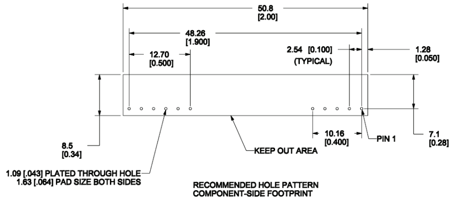
Module Layout – Back view
