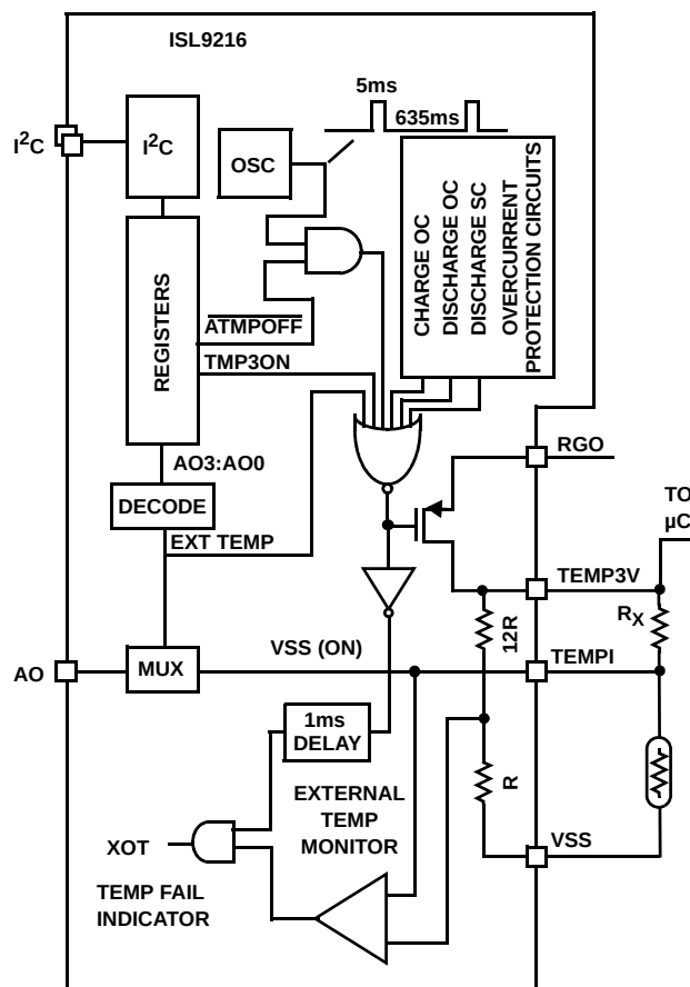
FIGURE 5. EXTERNAL TEMPERATURE MONITORING AND CONTROL (ISL9216 ONLY)
