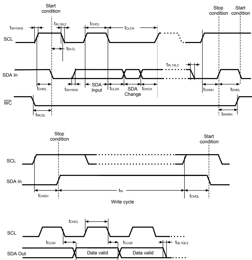
Figure 17. AC waveforms
