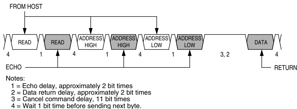
Figure 8-5. Read Transaction
