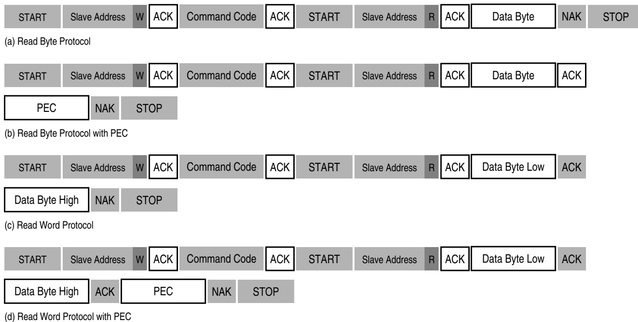
Figure 14-17. Read Byte/Word
