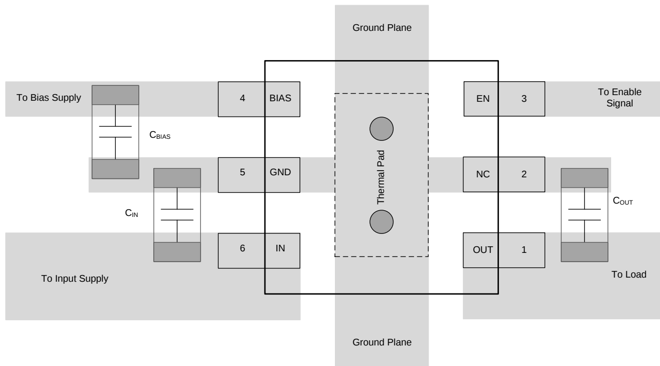
Figure 33. Recommended Layout
