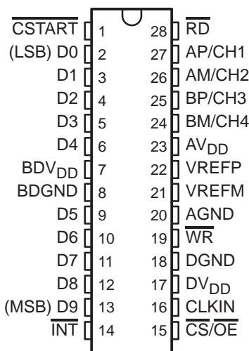
DW OR PW PACKAGE (TOP VIEW)
