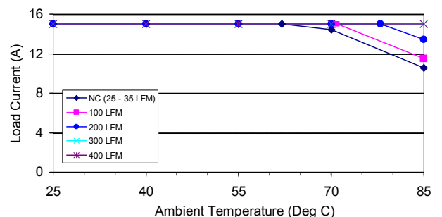
Figure 28. EMS15DE, V_{in} = 36 VDC
