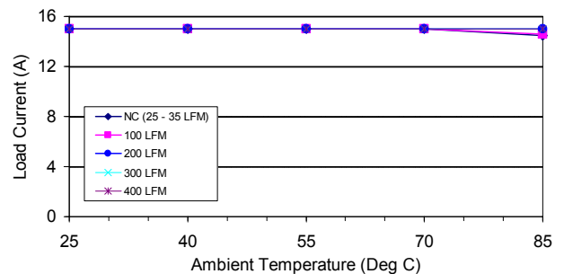
Figure 27. EMS15DE, V_{in} = 24 VDC
