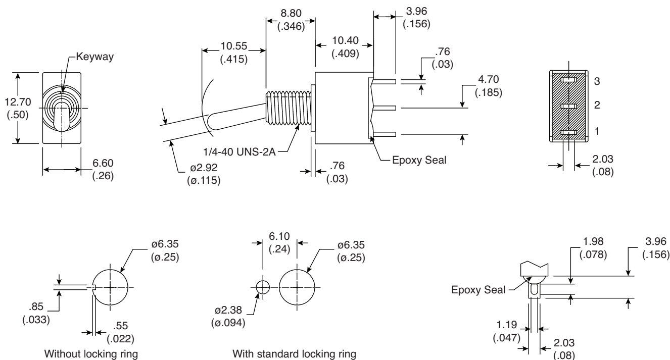
Panel Mounting
