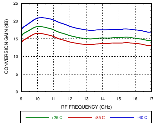
Conversion Gain, USB vs. Temperature
