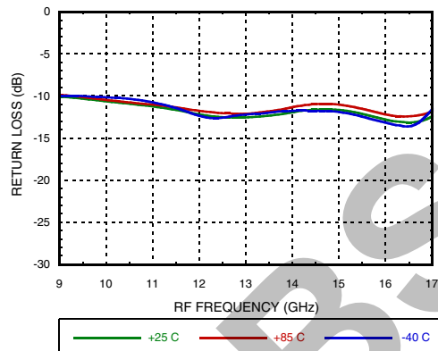
RF Return Loss vs. Temperature
