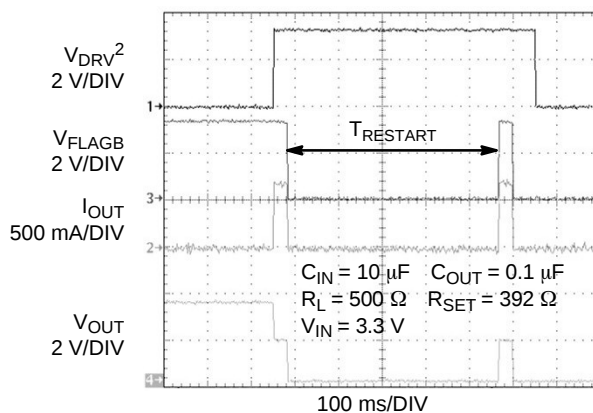
Figure 17. T_{RESTART} Response
