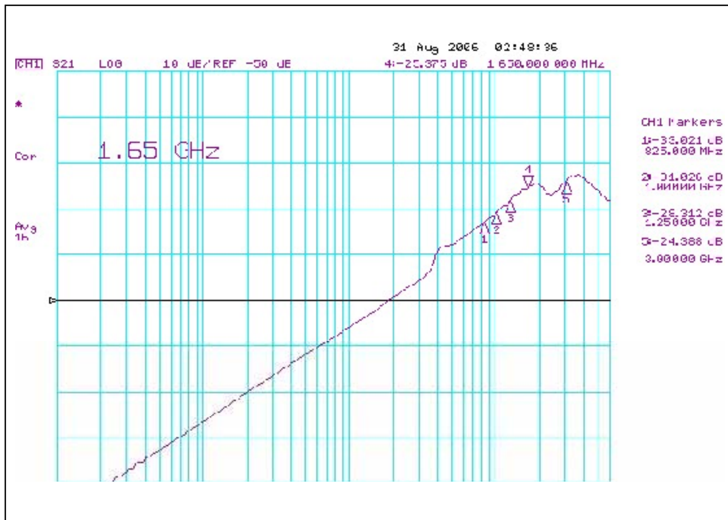
Fig 3. Crosstalk
