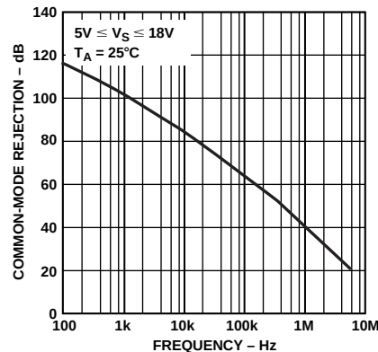
Figure 17. Common-Mode Rejection vs. Frequency
