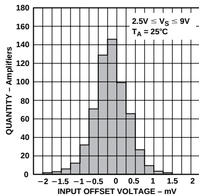
Figure 11. Input Offset Voltage Distribution
