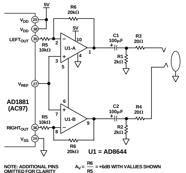
Figure 28. A PC-99-Compliant Headphone/Speaker Amplifier with Gain
