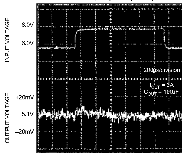
Line Transient Response with 3A Load, 100μF Output Capacitance
