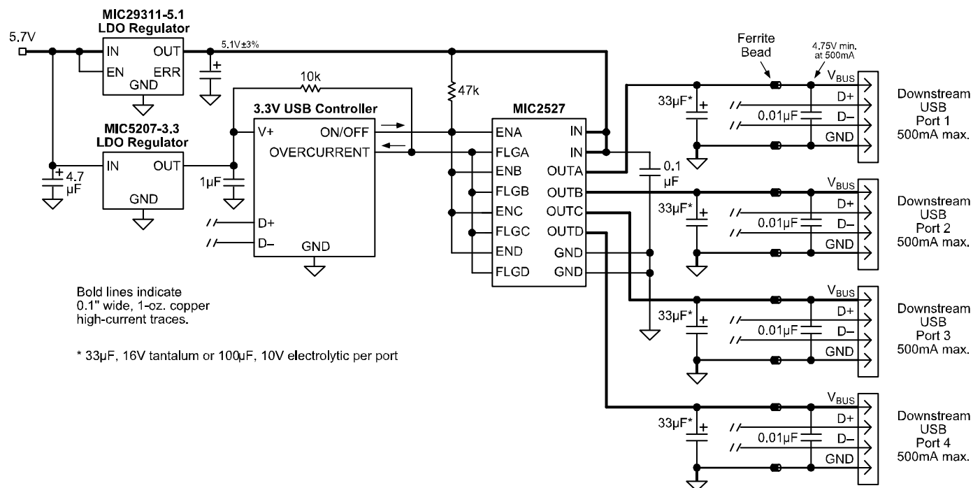
Figure 2. 4-Port Self-Powered Hub
