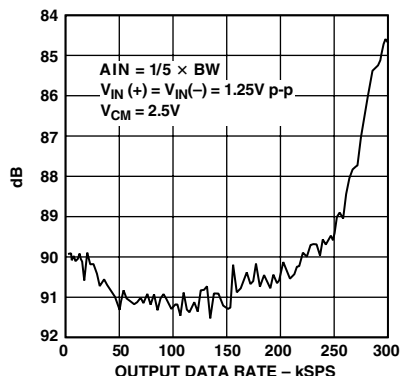
TPC 5. S/(N+D) vs. Output Sample Rate
