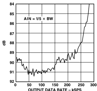
TPC 2. S/(N+D) vs. Output Sample Rate
