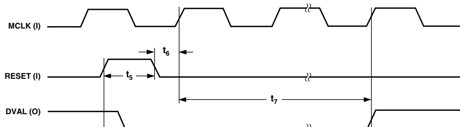
Figure 3. Data Timing
