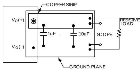
Figure 61. Input Reflected Ripple Current Test Setup.
