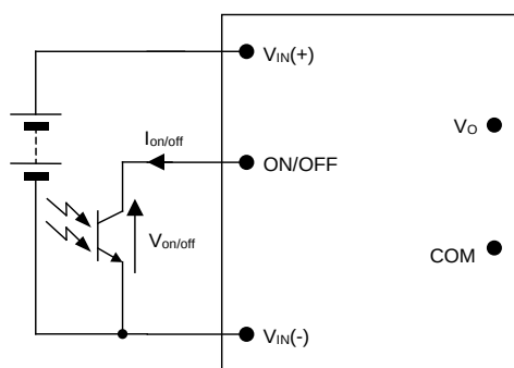
Figure 64. Remote On/Off Implementation.
