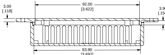
SECTION C-C
