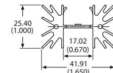
VIEW A-A SINGLE HEAT SINK DEVICE
