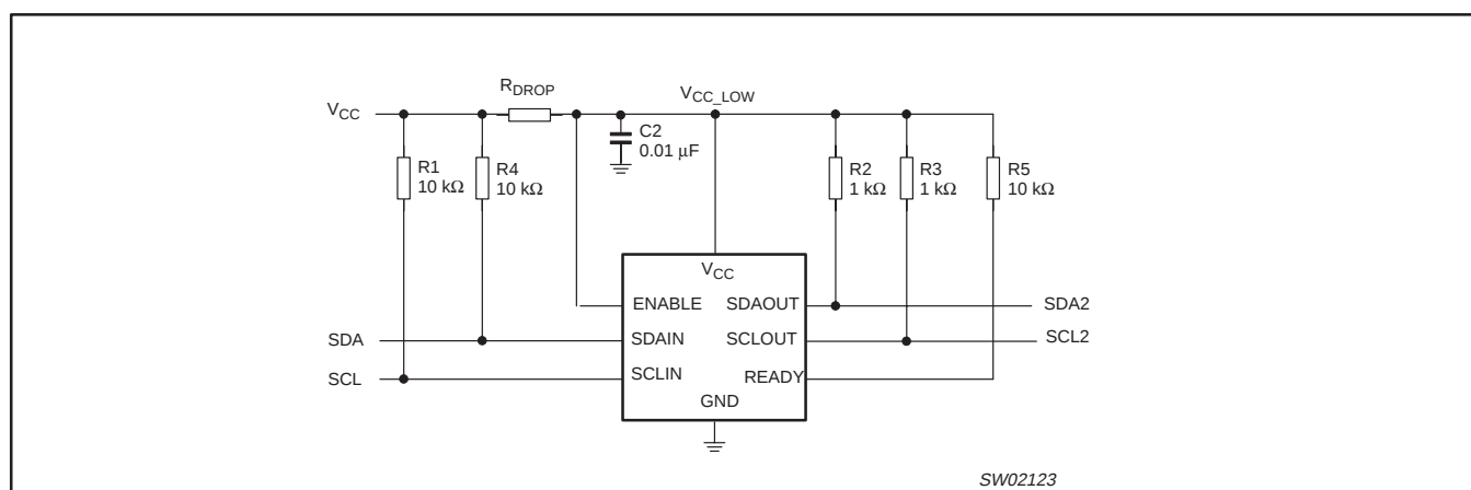
Figure 12. System with disparate V CC voltages
