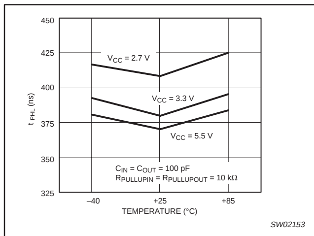
Figure 15. Input-output t_{PHL} versus Temperature.
