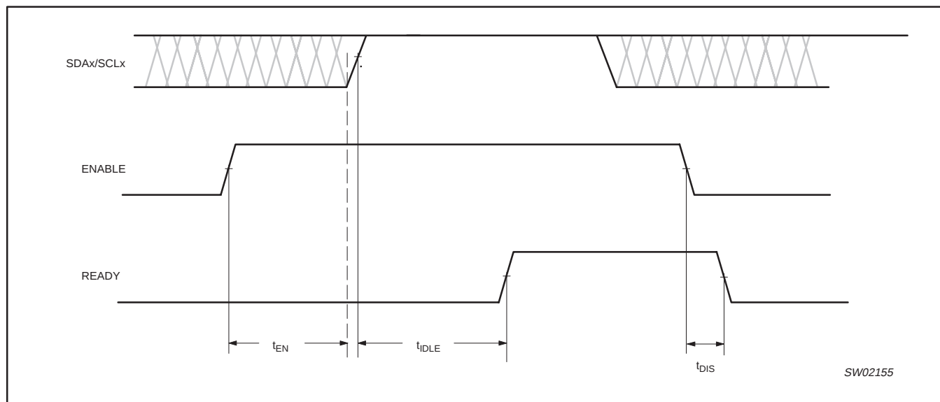
Figure 17. Timing for t_{\text{ENABLE}} , t_{\text{IDLE}} , and t_{\text{DISABLE}}
