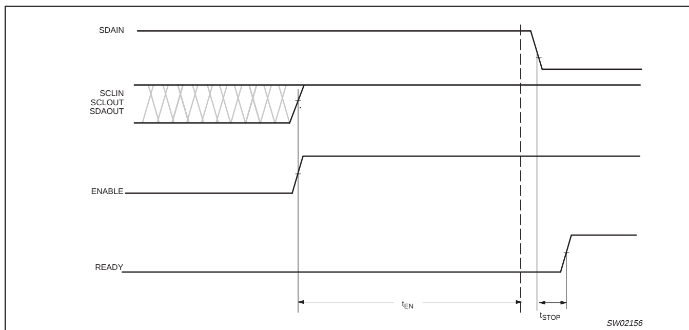
Figure 18. t_{\text{STOP}} that can occur after t_{\text{ENABLE}}
