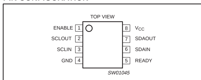
Figure 1. Pin configuration.
