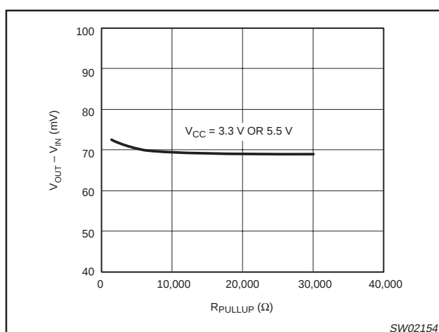
Figure 16. Connection circuitry V_{OUT} - V_{IN} .
