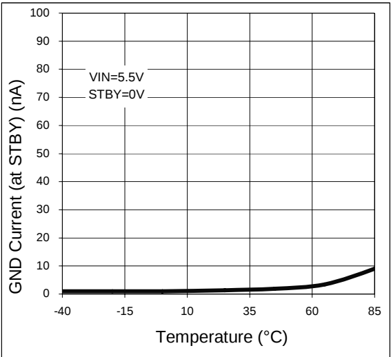
Figure 83. GND Current (at STBY) vs. Temperature
