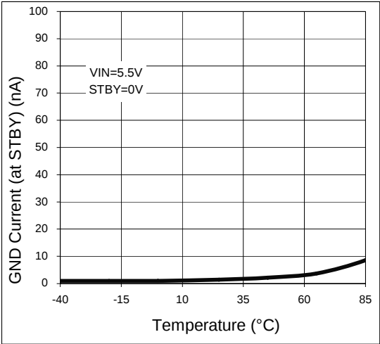
Figure 35. GND Current (at STBY) vs. Temperature
