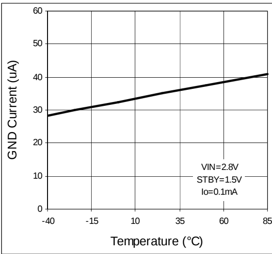
Figure 10. GND Current vs. Temperature
