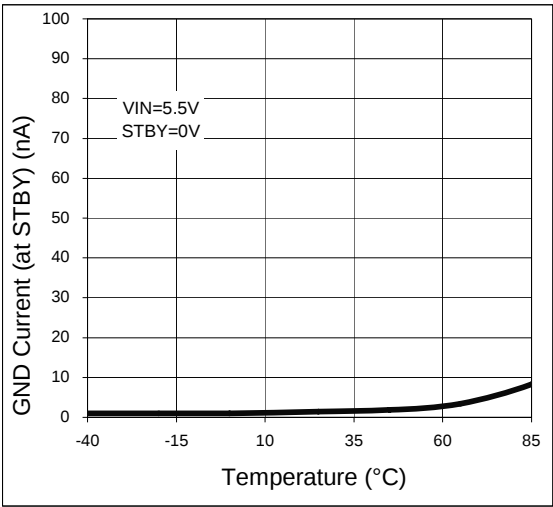
Figure 59. GND Current(at STBY) vs. Temperature
