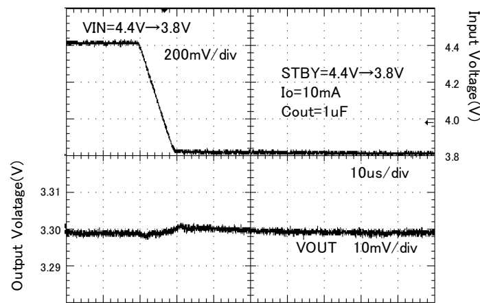
Figure 97. Line response ( Vin= 4.4 V → 3.8 V)
