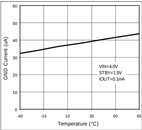
Figure 57. GND Current vs. Temperature
