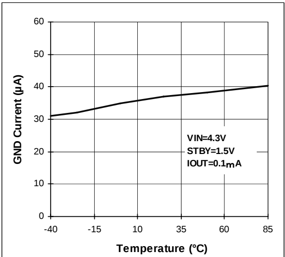
Figure 81. GND Current vs. Temperature
