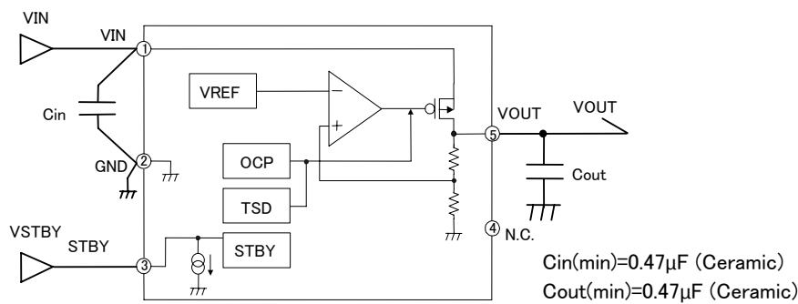
Figure 2. Block diagram
