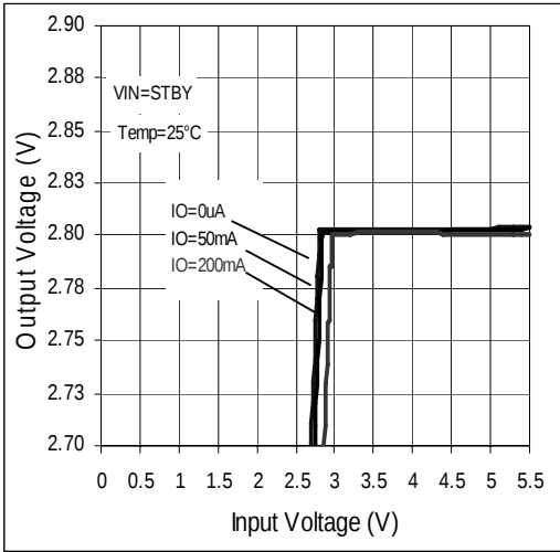
Figure 27. Line Regulation
