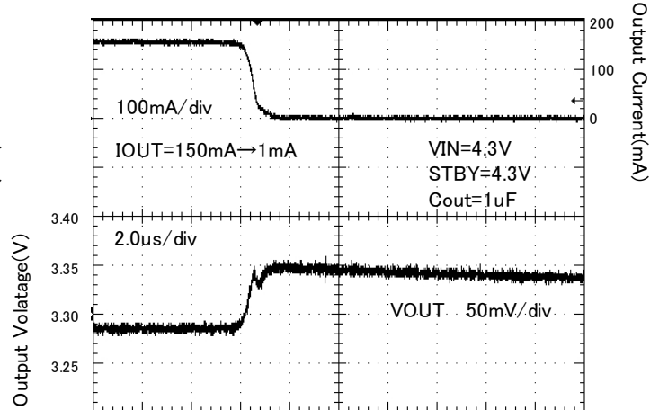
Figure 95. Load response ( Iout = 150mA → 1mA)
