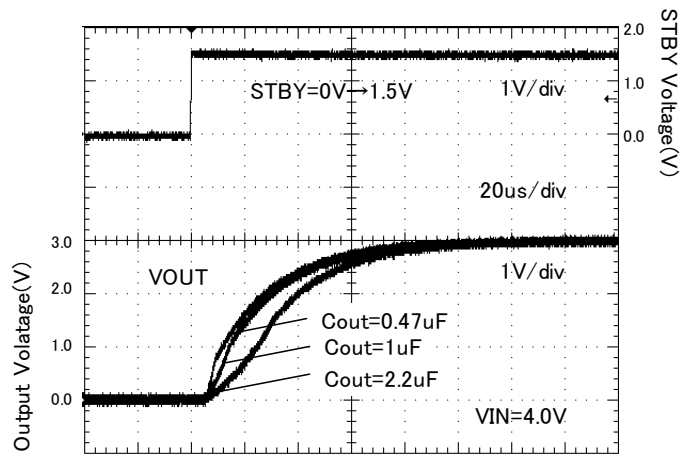
Figure 66. Startup time ( Rout = none )
