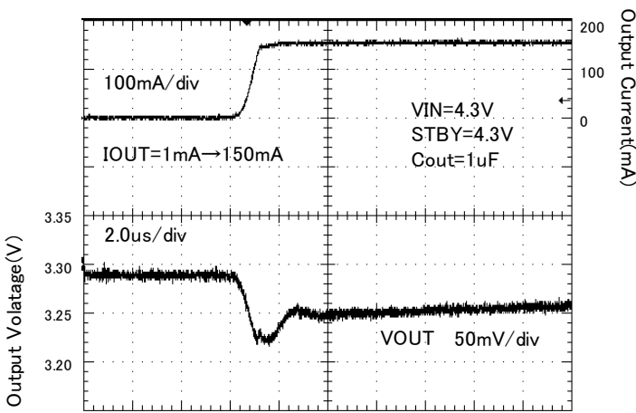
Figure 94. Load response ( Iout = 1mA → 150mA)
