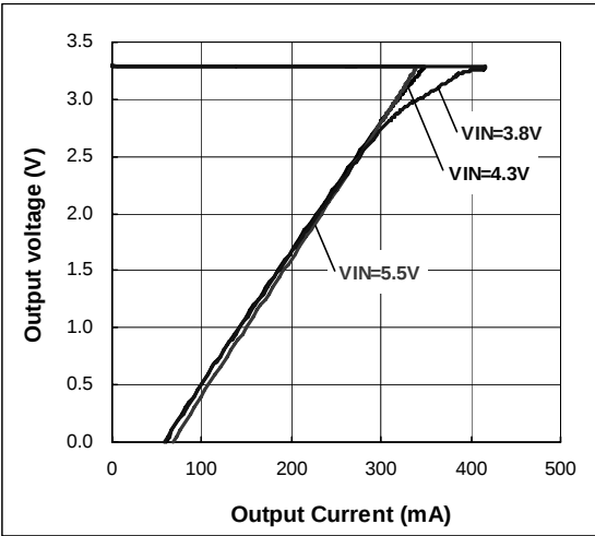
Figure 79. OCP Threshold
