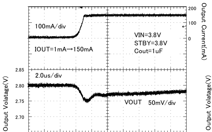
Figure 46. Load response ( I_{out} = 1\text{mA} \rightarrow 150\text{mA} )
