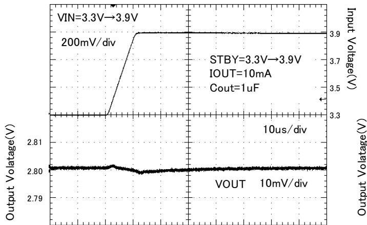
Figure 48. Line response ( V_{in} = 3.3\text{V} \rightarrow 3.9\text{V} )
