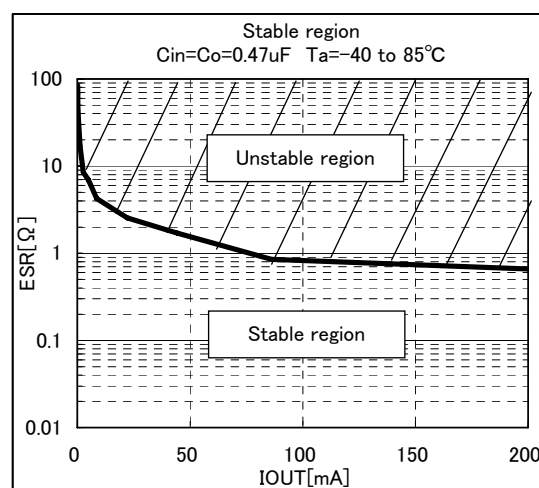
Figure 99. Stability area characteristics (Example)
