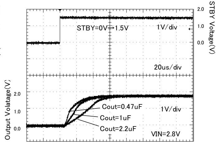
Figure 19. Startup time ( Rout = 9 ohm )
