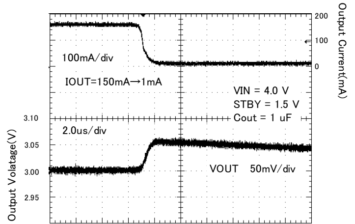
Figure 71. Load response ( I_{out} = 150\text{mA} \rightarrow 1\text{mA} )
