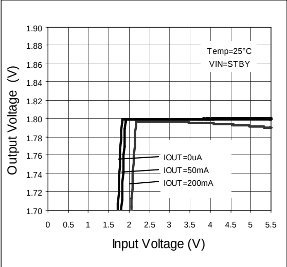
Figure 4. Line Regulation
