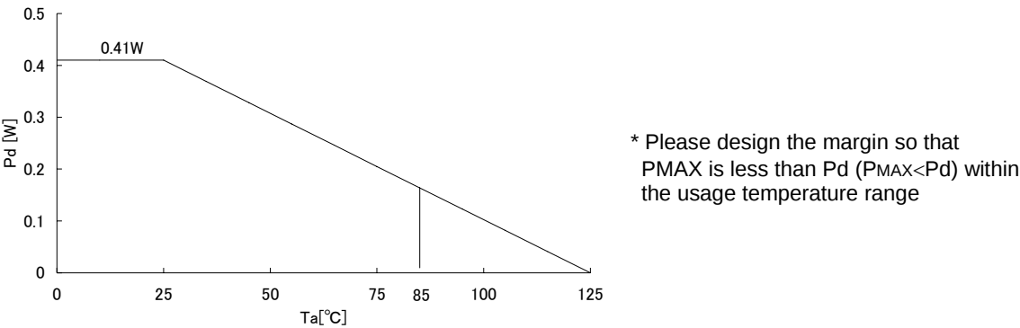
Figure 100. UCSP50L1(BUXXSA4WGWL) Power dissipation heat reduction characteristics (Reference)
