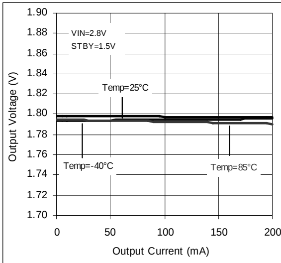
Figure 6. Load Regulation
