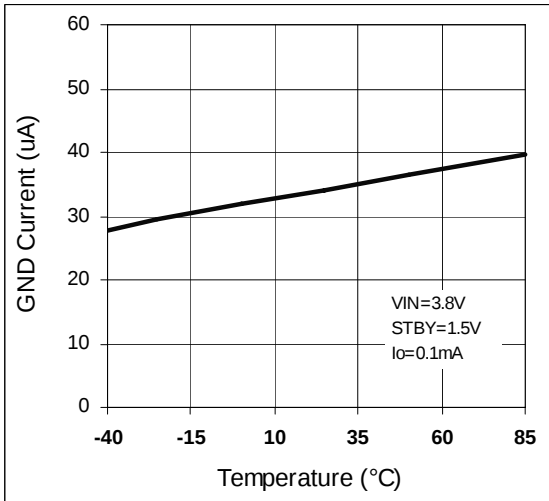
Figure 33. GND Current vs. Temperature
