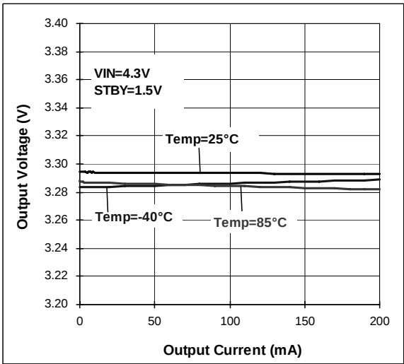
Figure 77. Load Regulation
