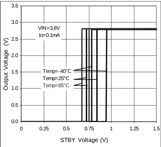
Figure 34. STBY Threshold
