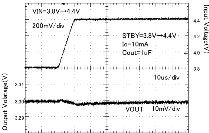
Figure 96. Line response ( Vin= 3.8 V → 4.4 V)
