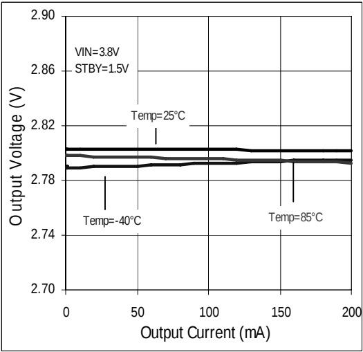
Figure 29. Load Regulation
