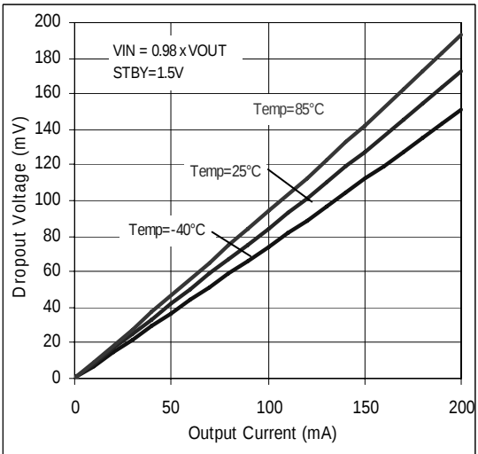
Figure 37. Dropout Voltage vs. Output Current
