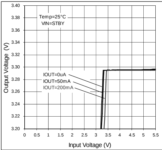
Figure 75. Line Regulation
