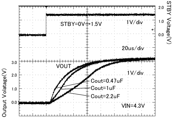
Figure 91. Startup time ( Rout = 16.5 ohm )
