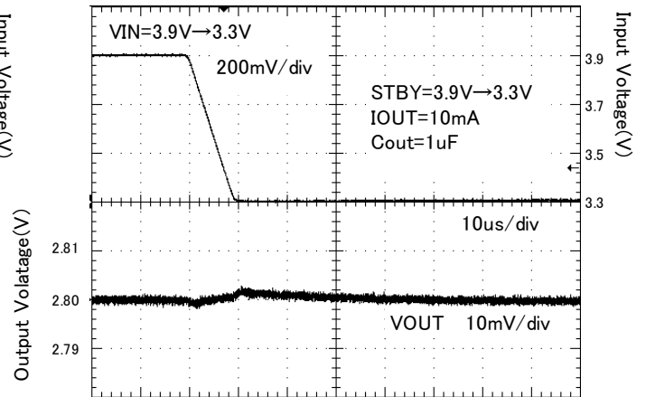
Figure 49. Line response ( V_{in} = 3.9\text{V} \rightarrow 3.3\text{V} )
