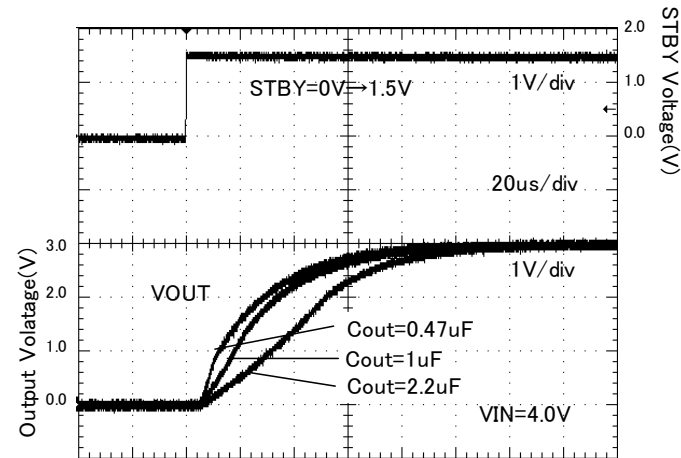
Figure 67. Startup time ( Rout = 15 ohm )
