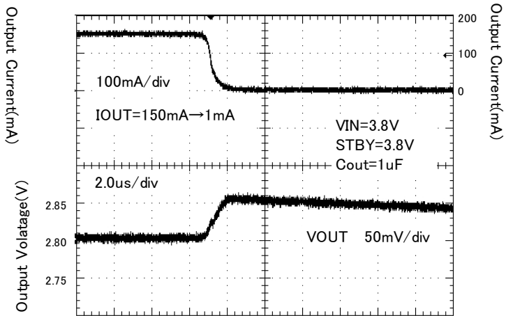
Figure 47. Load response ( I_{out} = 150\text{mA} \rightarrow 1\text{mA} )
