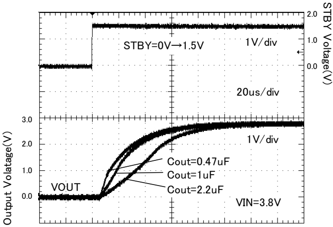
Figure 43. Startup time ( Rout = 14 ohm )
