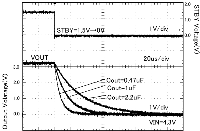
Figure 93. Discharge time ( Rout = 16.5 ohm )
