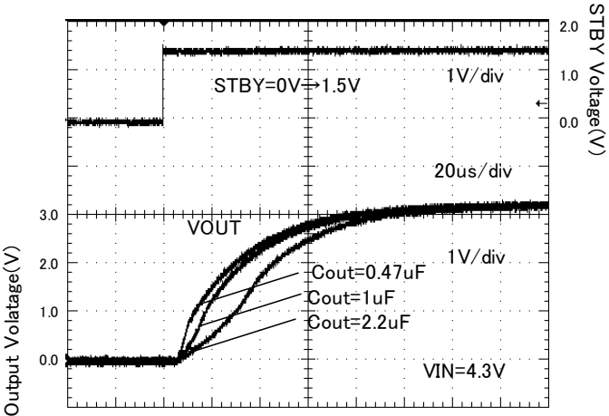
Figure 90. Startup time ( Rout = none )
