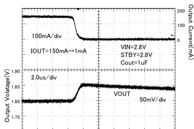
Figure 23. Load response ( Iout = 150mA → 1mA)
