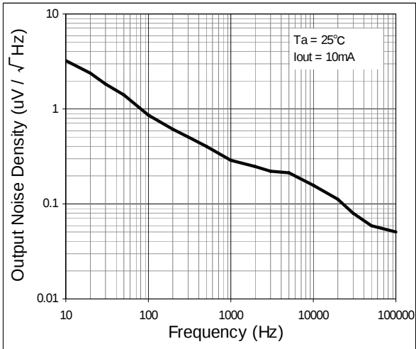
Figure 17. Output Noise Density vs. Frequency
