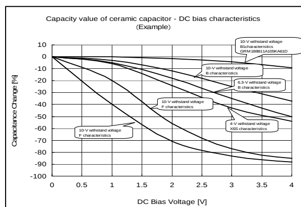
Figure 98. Capacity-bias characteristics
