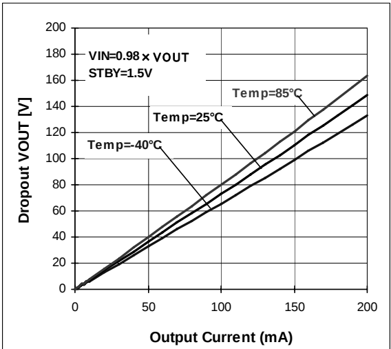
Figure 85. Dropout Voltage vs. Output Current
