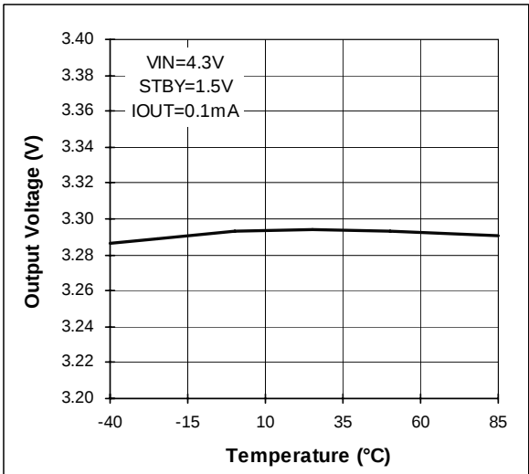
Figure 80. Output Voltage vs. Temperature
