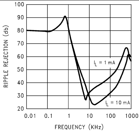
Figure 7. Ripple Rejection
