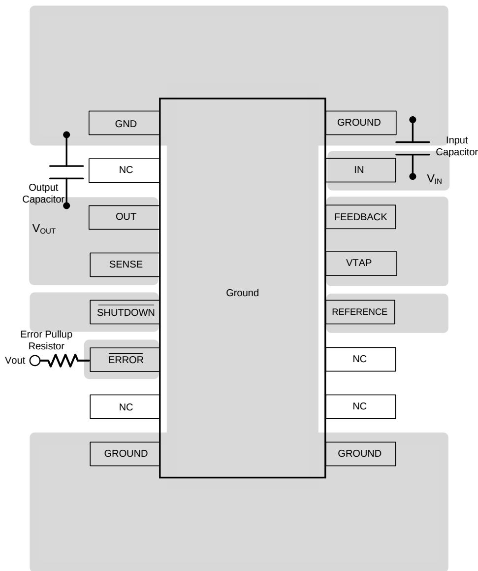
Figure 46. Layout Schematic
