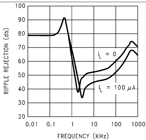
Figure 9. Ripple Rejection
