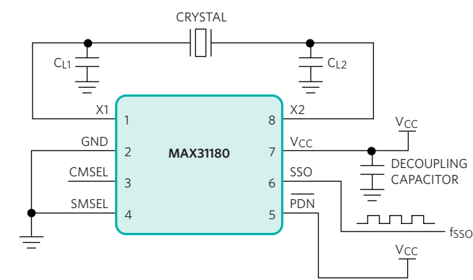
WITH PDN CONNECTED TO VCC, SMSEL CONNECTED TO GND AND CMSEL OPEN, THE DEVICE IS IN NORMAL OPERATION WITH 2x CLOCK MULTIPLICATION, AND SPREAD-SPECTRUM MAGNITUDE OF ±0.5%.
