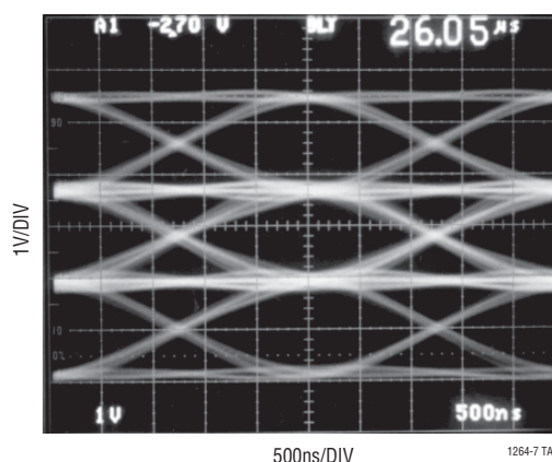
4-Level PAM Eye Diagram
