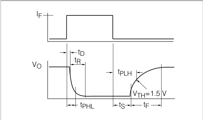
Figure 10. Switching waveform
