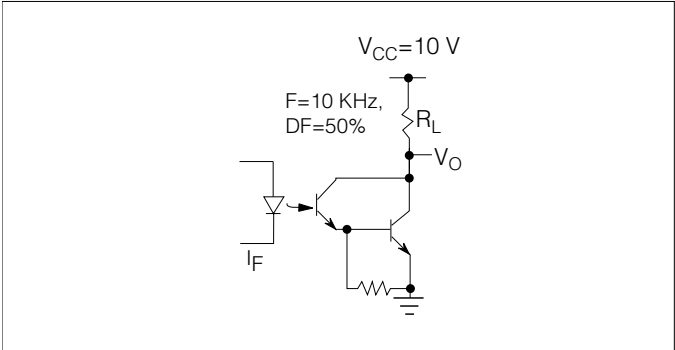
Figure 11. Switching schematic
