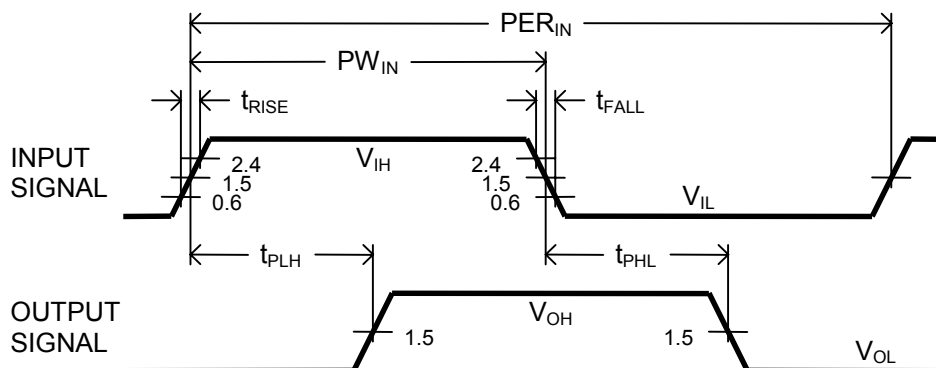
Figure 7: Timing Diagram
