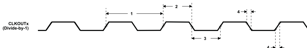
Figure 8-16. CLKOUTx Timing
