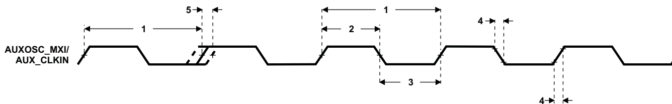
Figure 8-13. AUX_MXI/AUX_CLKIN Timing
