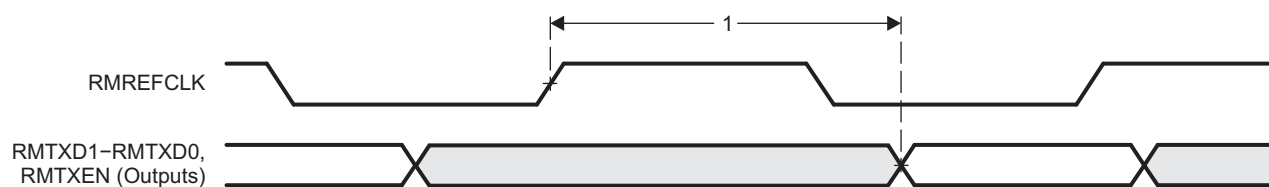
Figure 9-15. EMAC Transmit Interface Timing RMII Operation
