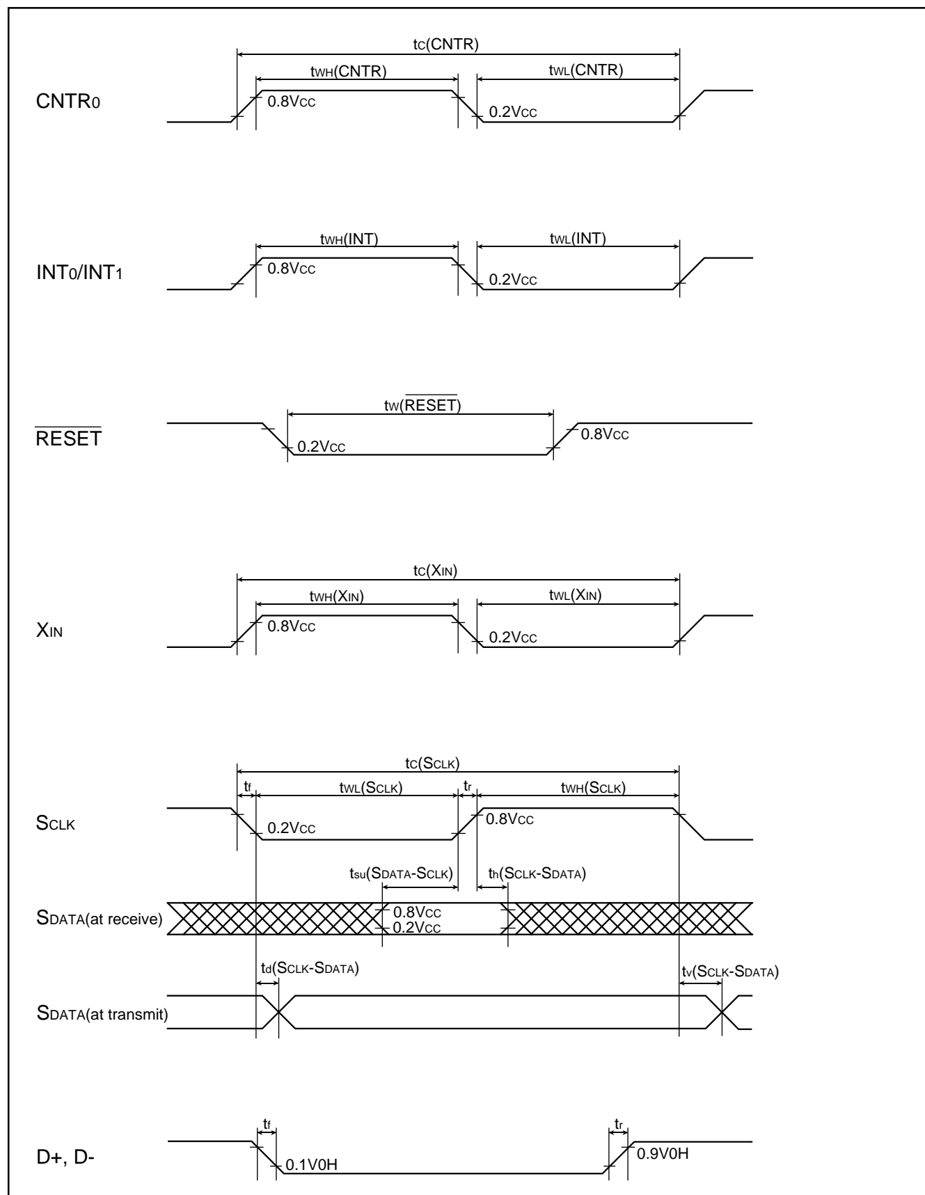
Fig. 50 Timing chart
