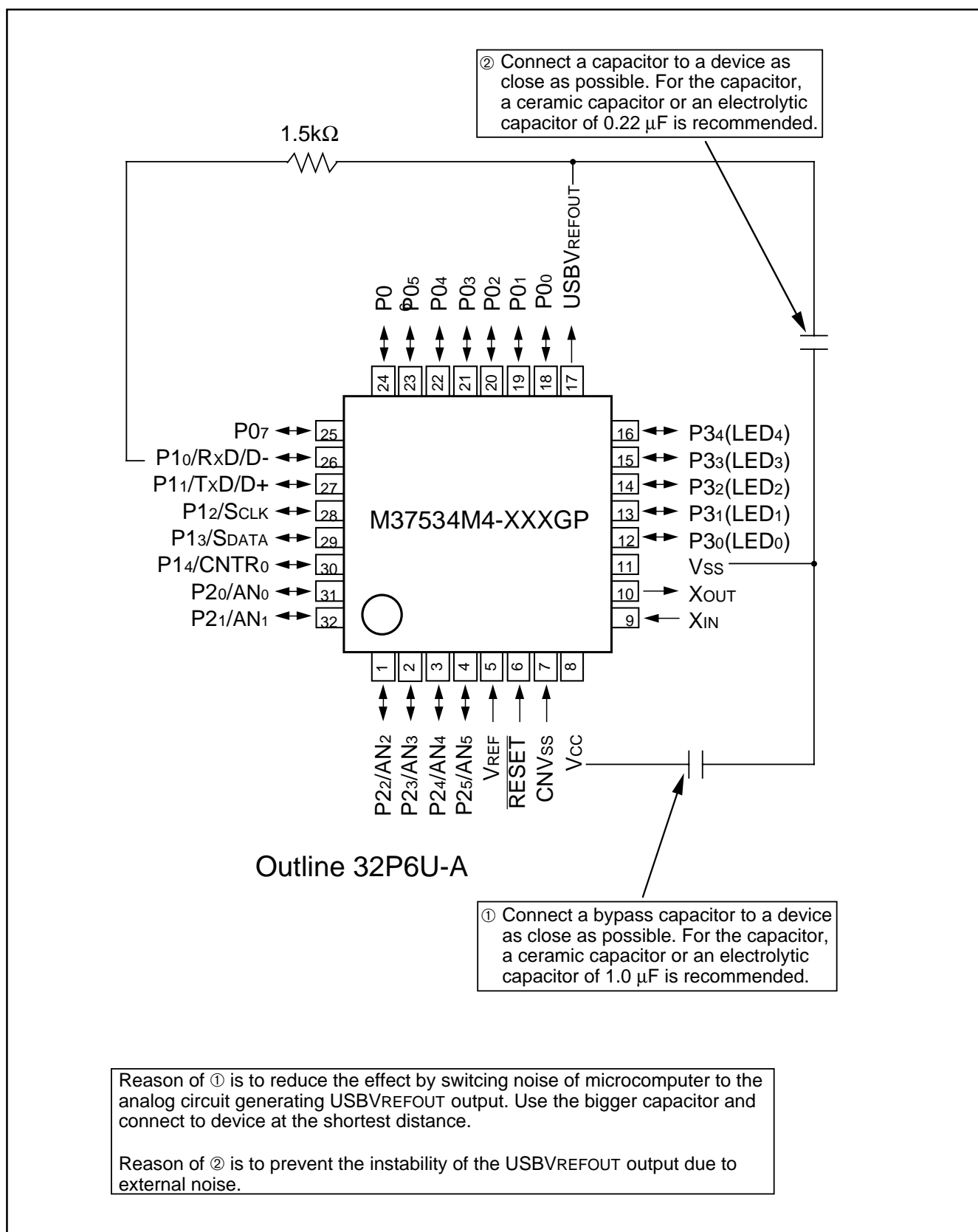
Fig. 52 Handling of V CC , USBV REFOUT pins of M37534M4-XXXGP
