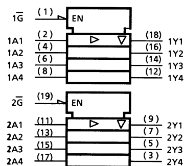
TC74HC244A
