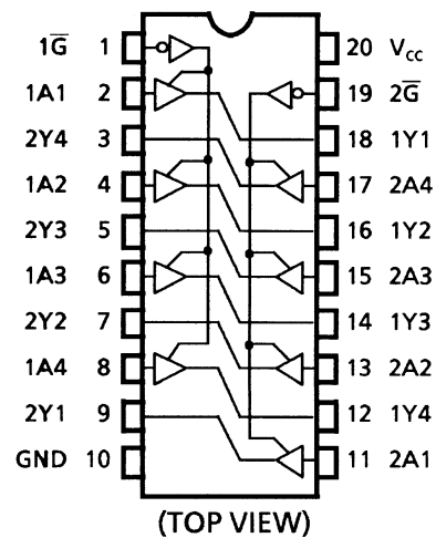
TC74HC244A
