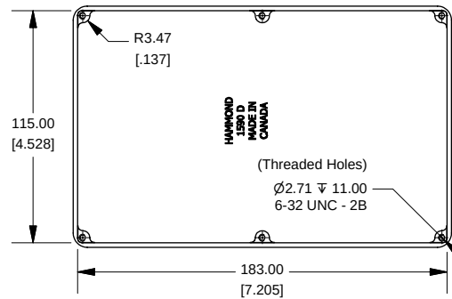
Top View Looking Inside Box
