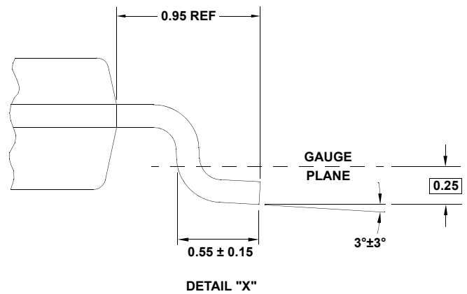
DETAIL "X"
