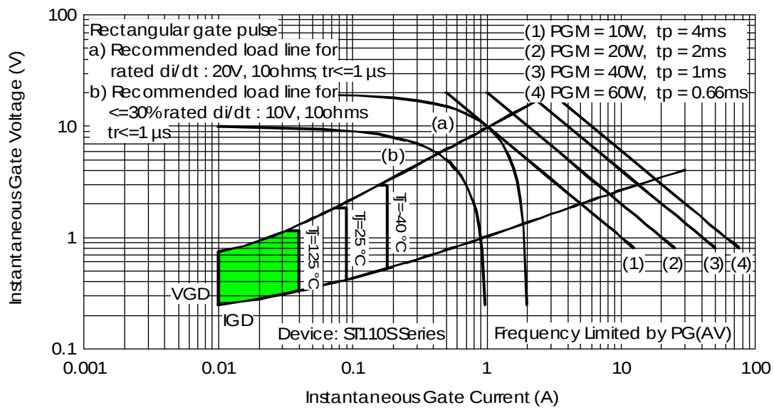
Fig. 9 - Gate Characteristics
