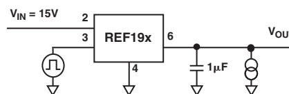
TPC 11b. \overline{\text{SLEEP}} Response Time Measurement Circuit
