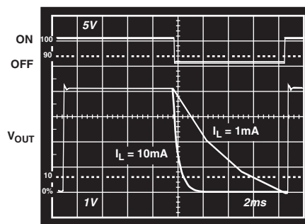
TPC 11a. \overline{\text{SLEEP}} Response Time
