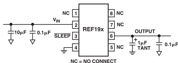
Figure 2. Basic Voltage Reference Configuration
