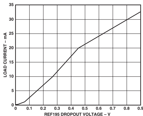
TPC 13. Dropout Voltage vs. Load Current
