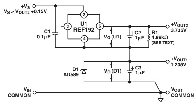
Figure 7. Stacking Voltage References with the REF19x
