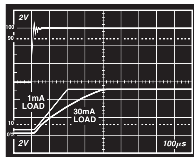
TPC 10a. Power ON Response Time
