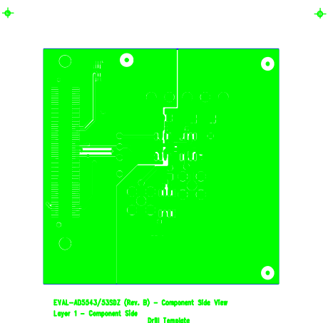
Figure 8. Top Side
