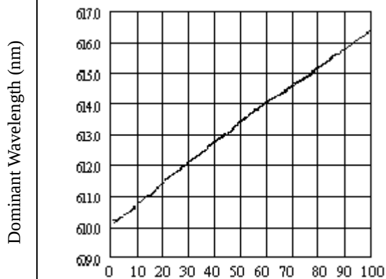
Dominant Wavelength vs. Forward Current (Ta=25°C)
