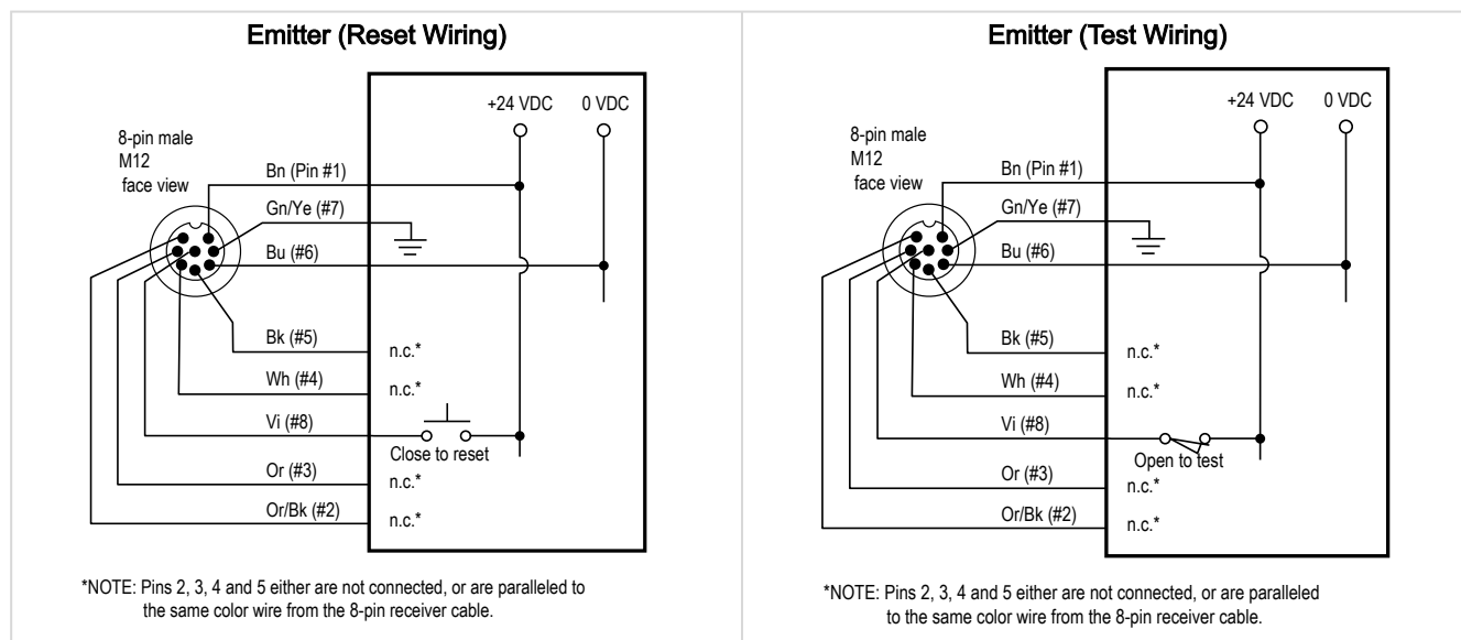
Figure 38. Emitter—Generic wiring
