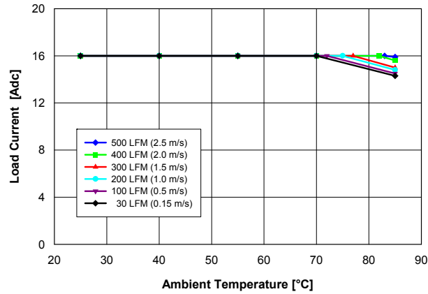
Fig. 1.8V.1: Available load current vs. ambient temperature and airflow rates for V_{out} = 1.8V converter mounted vertically with V_{in} = 12V , and maximum MOSFET temperature \leq 120^{\circ}C .
