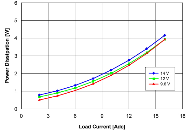
Fig. 2.0V.3: Power loss vs. load current and input voltage for V_{out} = 2.0V converter mounted vertically with air flowing at a rate of 200 LFM (1 m/s) and T_a = 25^{\circ}C .
