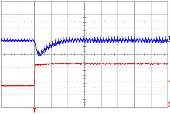
Fig. 5.0V.6: Output voltage response for V_{out} = 5.0V to positive load current step change from 8A to 16A with slew rate of 5A/\mu s at V_{in} = 12V . Top trace: output voltage (200mV/div.); Bottom trace: load current (5A/div.). C_o = 100\mu F ceramic. Time scale: 20μs/div.
