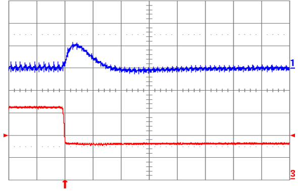
Fig. 2.5V.7: Output voltage response for V_{out} = 2.5V to negative load current step change from 16A to 8A with slew rate of -5A/\mu s at V_{in} = 12V . Top trace: output voltage (200mV/div.); Bottom trace: load current (5A/div.). C_o = 100\mu F ceramic. Time scale: 20\mu s /div.
