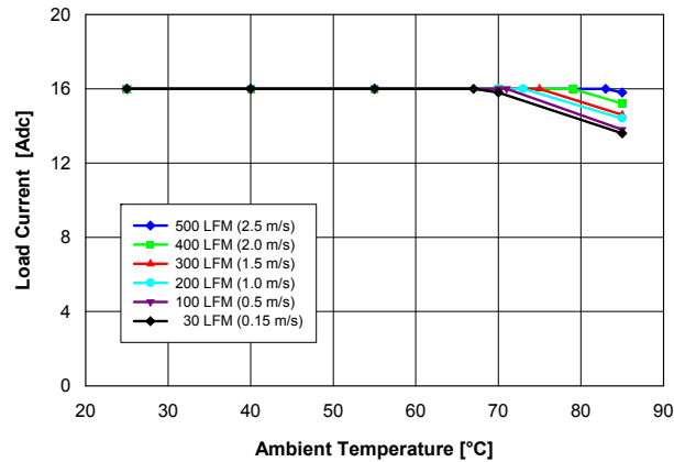
Fig. 3.3V.1: Available load current vs. ambient temperature and airflow rates for V out = 3.3V converter mounted vertically with V in = 12V, and maximum MOSFET temperature ≤ 120°C.
