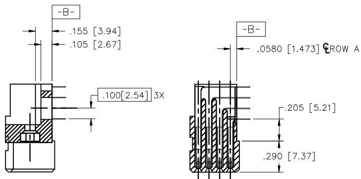
SECTION U-U
