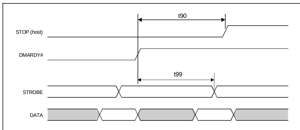
Figure 23-11. Ultra ATA Mode (Pausing a DMA Burst)
