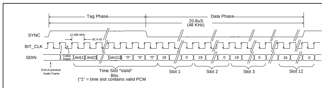
Figure 5-14. AC-Link Protocol
