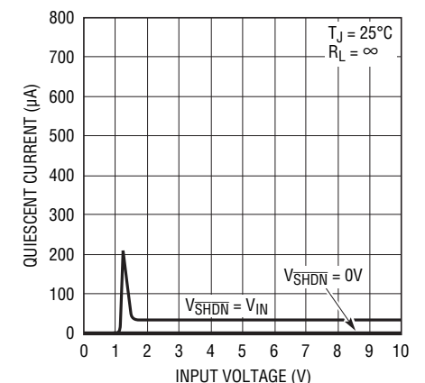
LT1962-1.5 Quiescent Current
