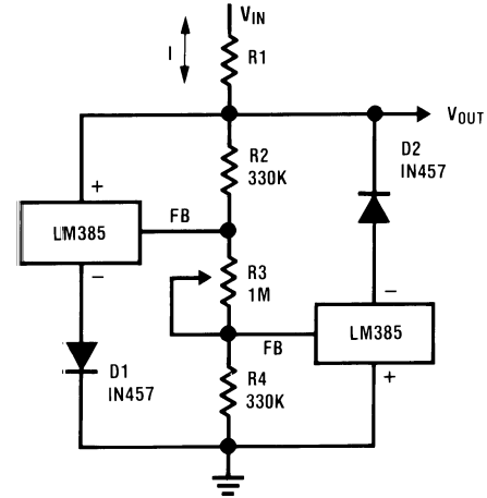
Figure 28. Bidirectional Adjustable Clamp \pm 2.4V to \pm 6V
