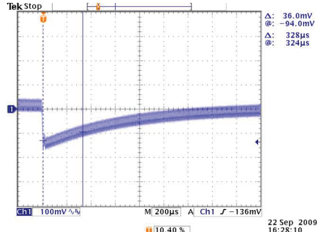
Output Ripple and Noise (Vin = 48V, Iout=0A, Cload=1μF ceramic II 10μF tantalum, Ta=+25°C., ScopeBW=20MHz)
