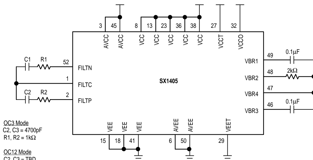
Figure 3. SX1405 Typical Operating Circuit
