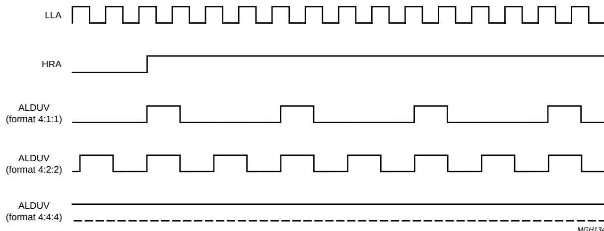
Fig.5 Timing of the signal ALDUV.
