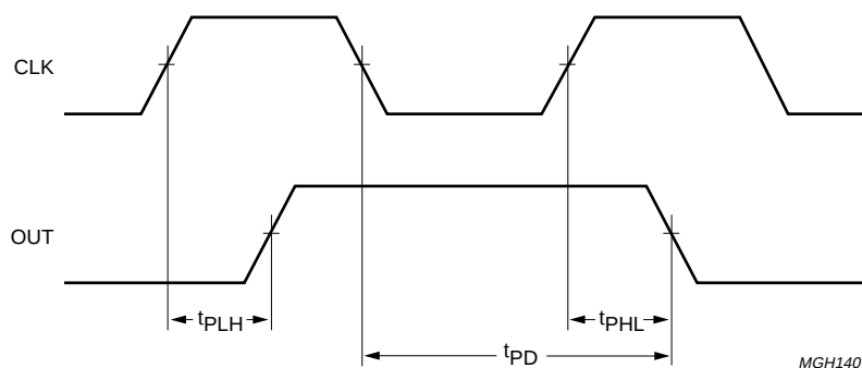
Fig.11 Timing diagram.
