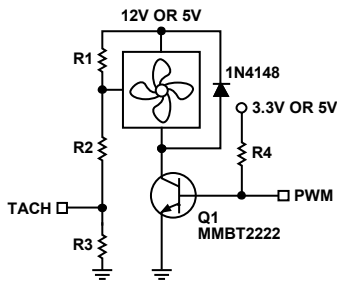
Figure 42. Planning for 3-Wire Fans on a PCB
