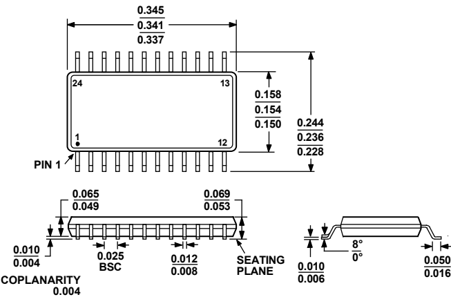
COMPLIANT TO JEDEC STANDARDS MO-137AE Figure 63. 24-Lead Shrink Small Outline Package [QSOP] (RQ-24) Dimensions shown in inches
