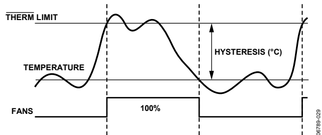
Figure 30. THERM Temperature Limit Operation
