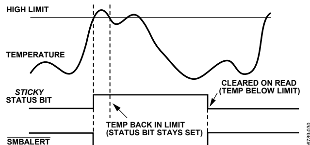
Figure 31. \overline{\text{SMBALERT}} and Status Bit Behavior
