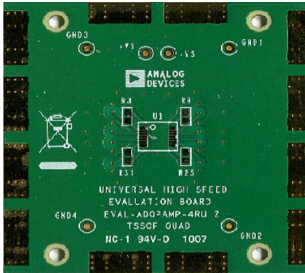
COMPONENT SIDE
