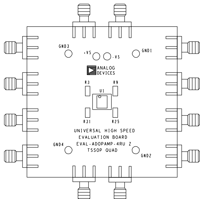
Figure 5. Board Assembly Drawing, Component Side
