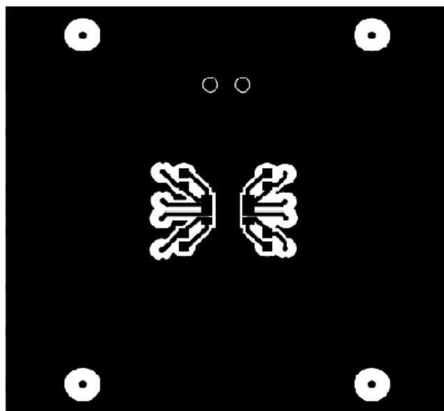
Figure 6. Board Layout Pattern, Component Side
