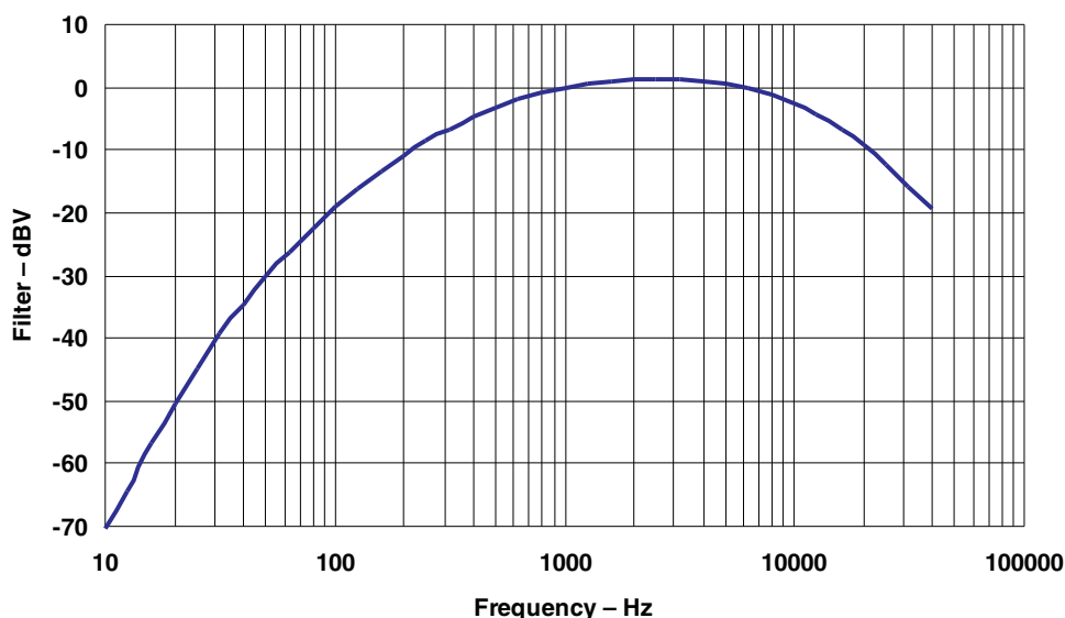
Figure 2. A-Weighted Filter
