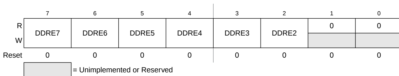
Figure 22-12. Port E Data Direction Register (DDRE)
